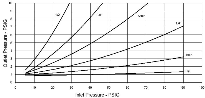
Relief Curves
