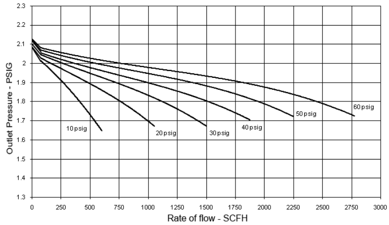
Relief Curves
