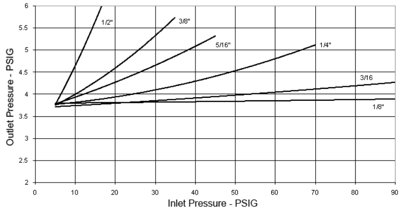
Relief Curves
