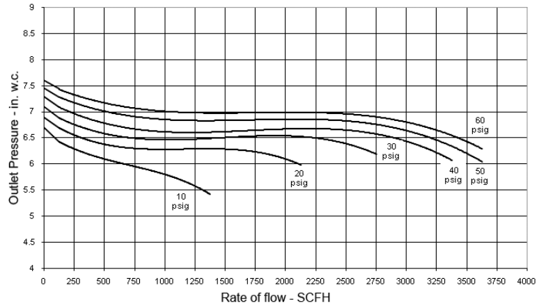
Performance Curves
