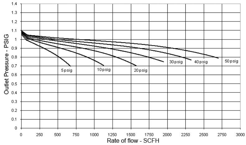
Relief Curves
