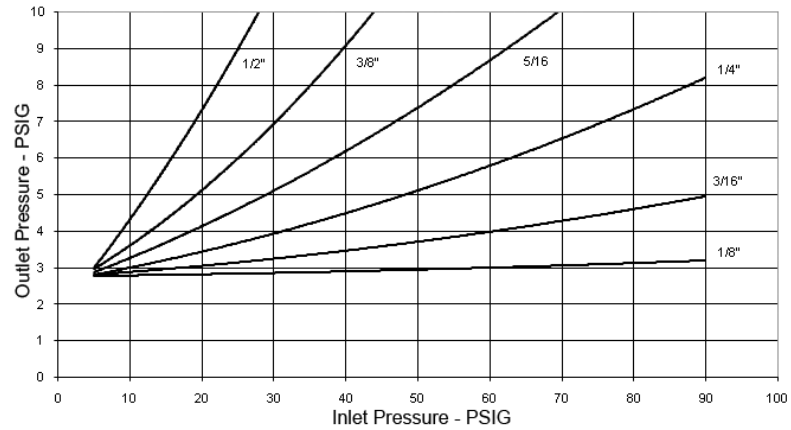
Relief Curves
