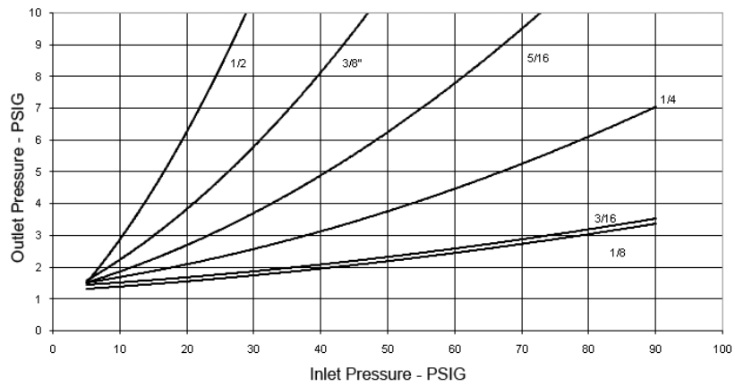
Relief Curves
